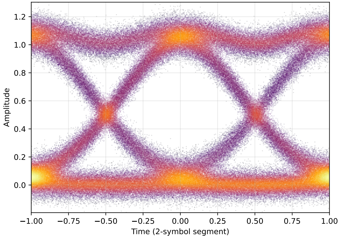
Eye Diagram (1024 traces)
